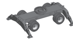
Standard-undercarriage Standard-Unterwagen
