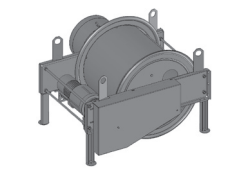
Cable drum Kabeltrommel
